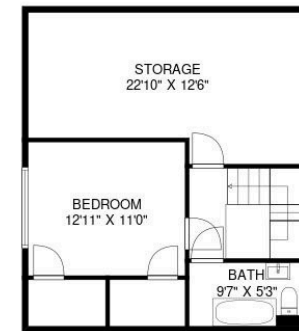
THIRD FLOOR
