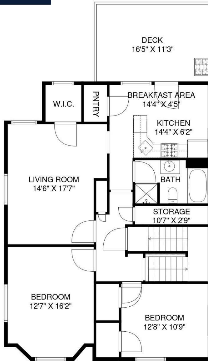
FIRST FLOOR
