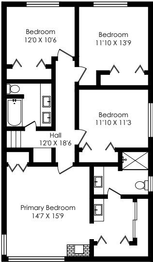
Upper Level
