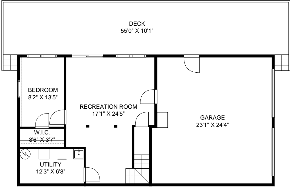
LOWER LEVEL
