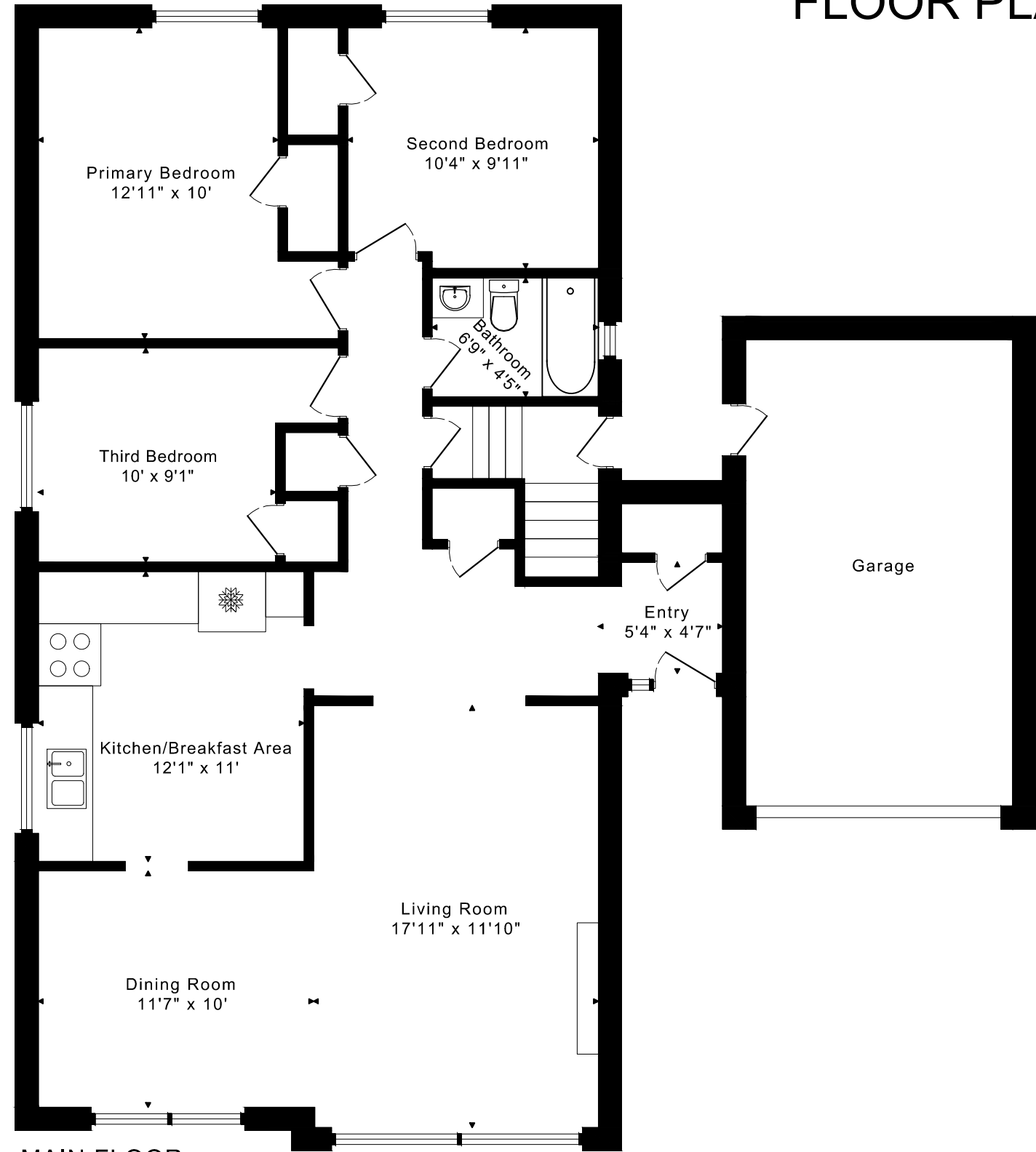
MAIN FLOOR 1275 SQUARE FEET
