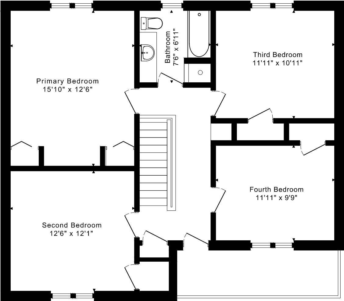
SECOND FLOOR 960 SQUARE FEET
