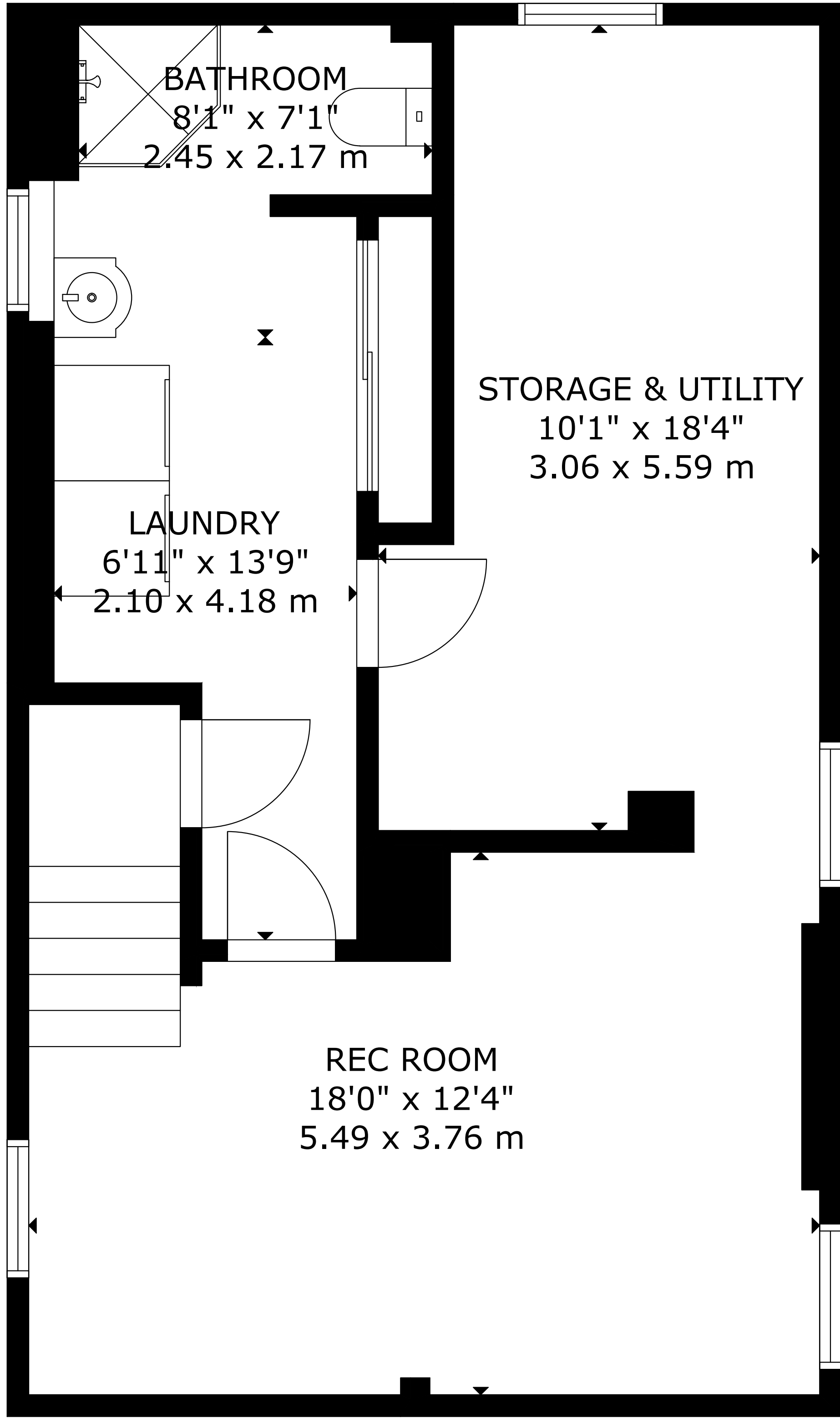
LOWER FLOOR
