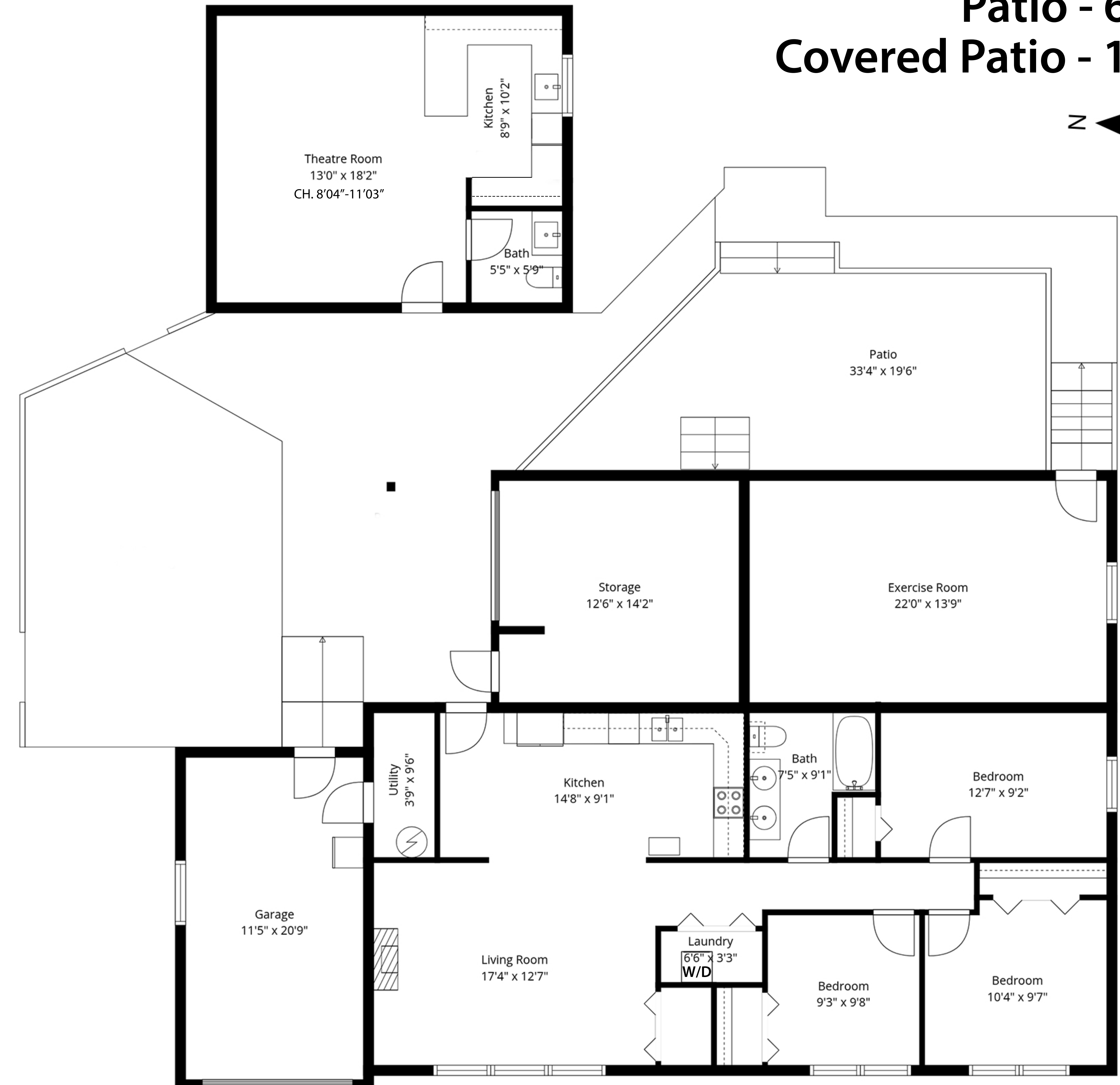
Lower Level - 1,935 Sq.Ft Ceiling Height - 7'2"
