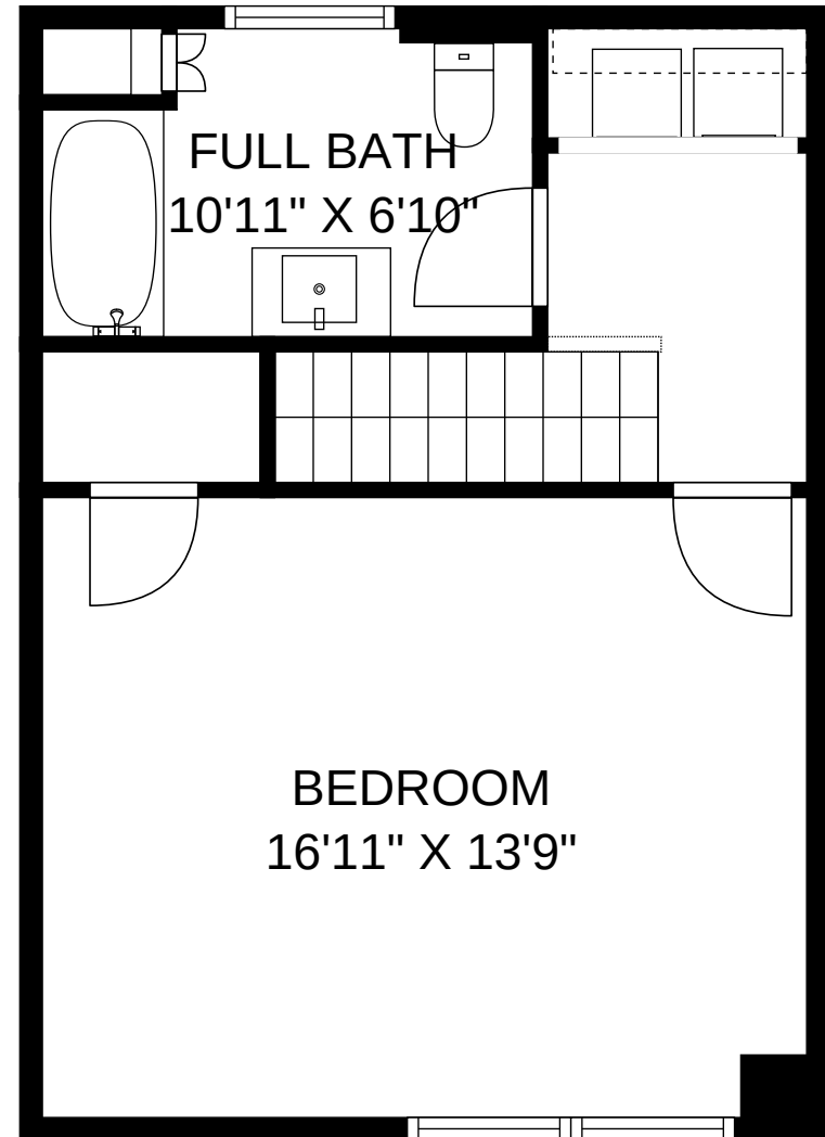
SECOND FLOOR
