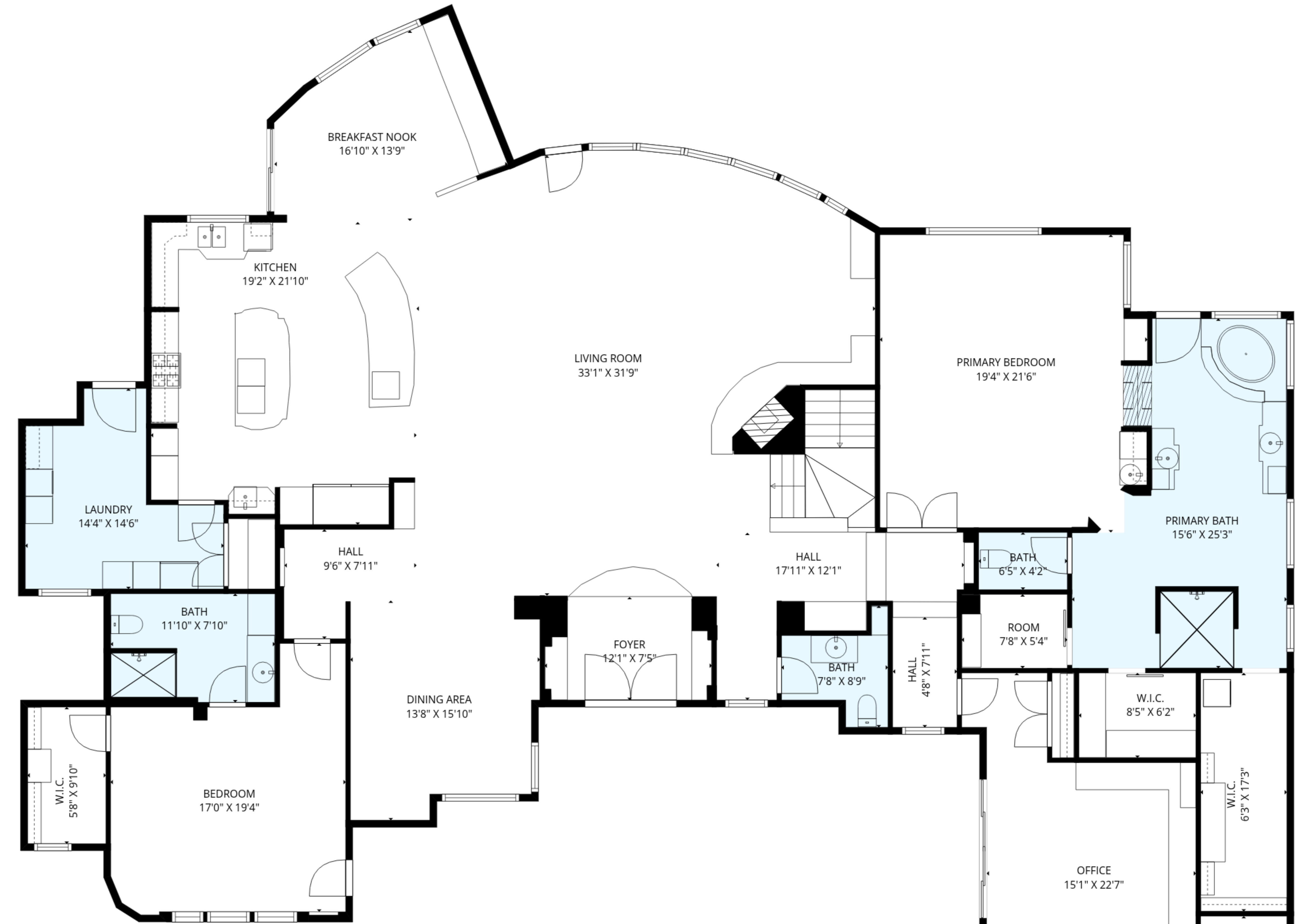
2ND FLOOR
