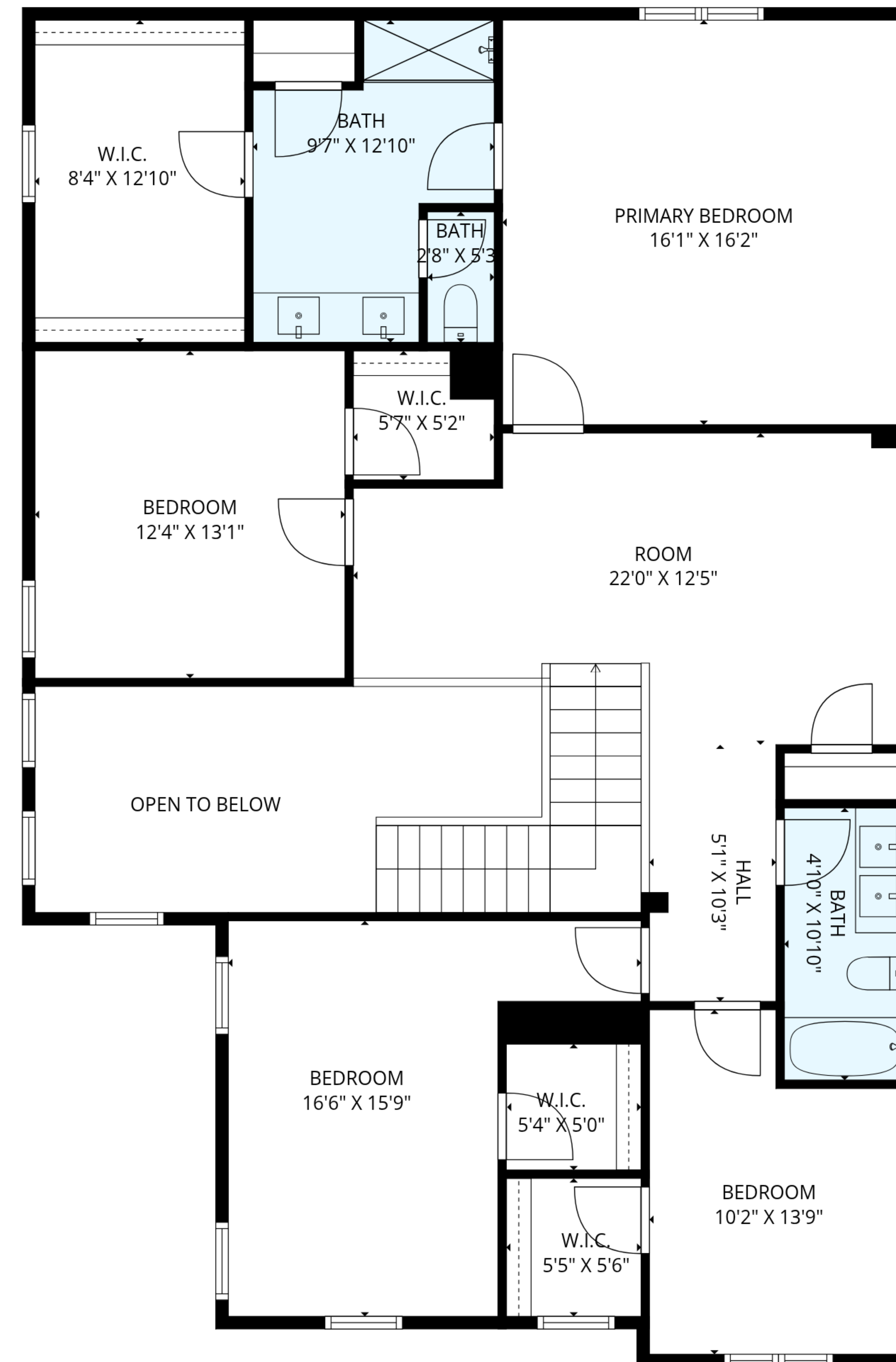
2ND FLOOR
