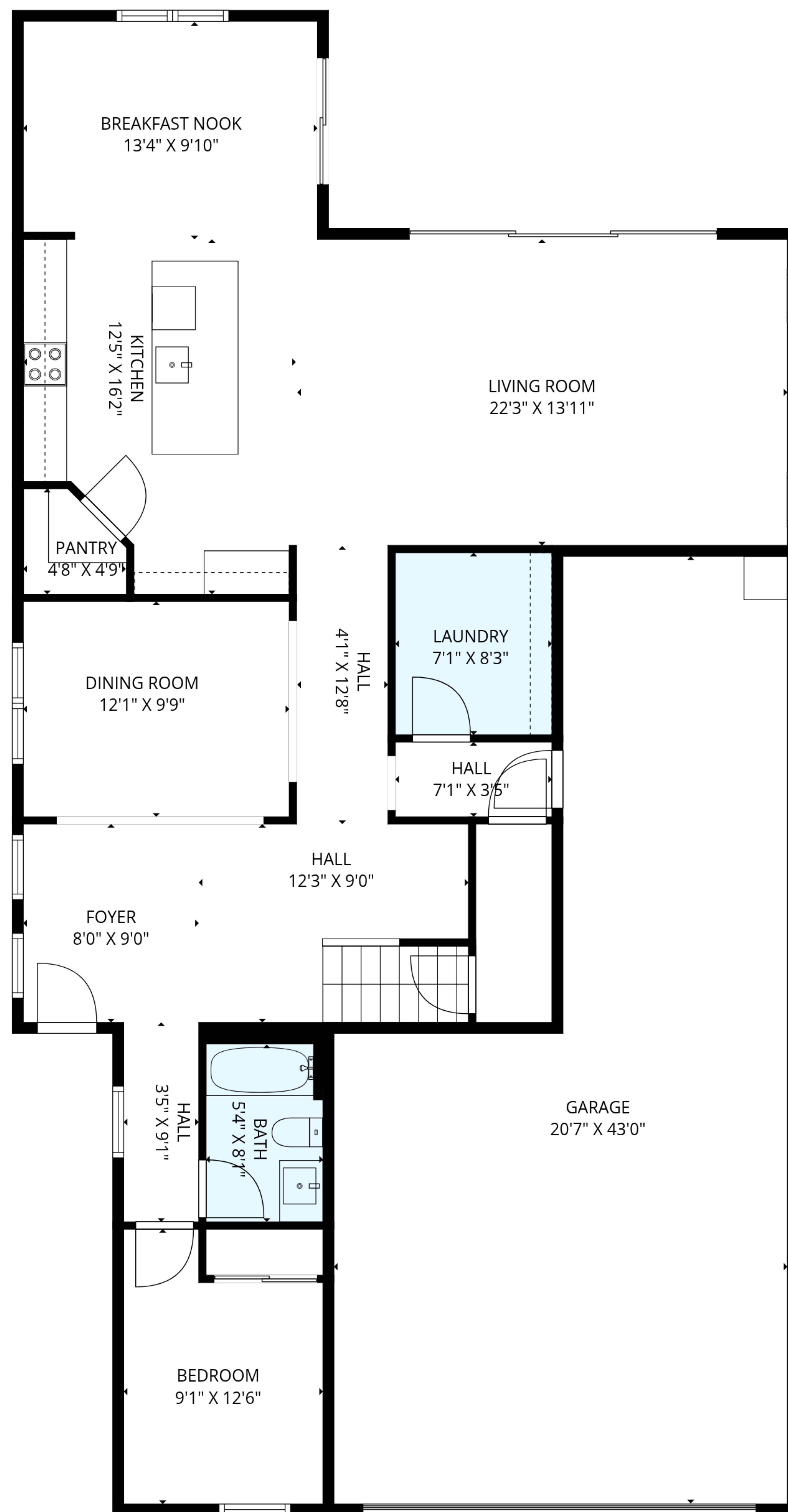
1ST FLOOR
