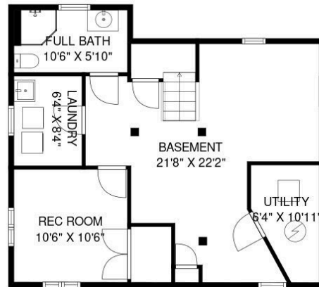
LOWER LEVEL
