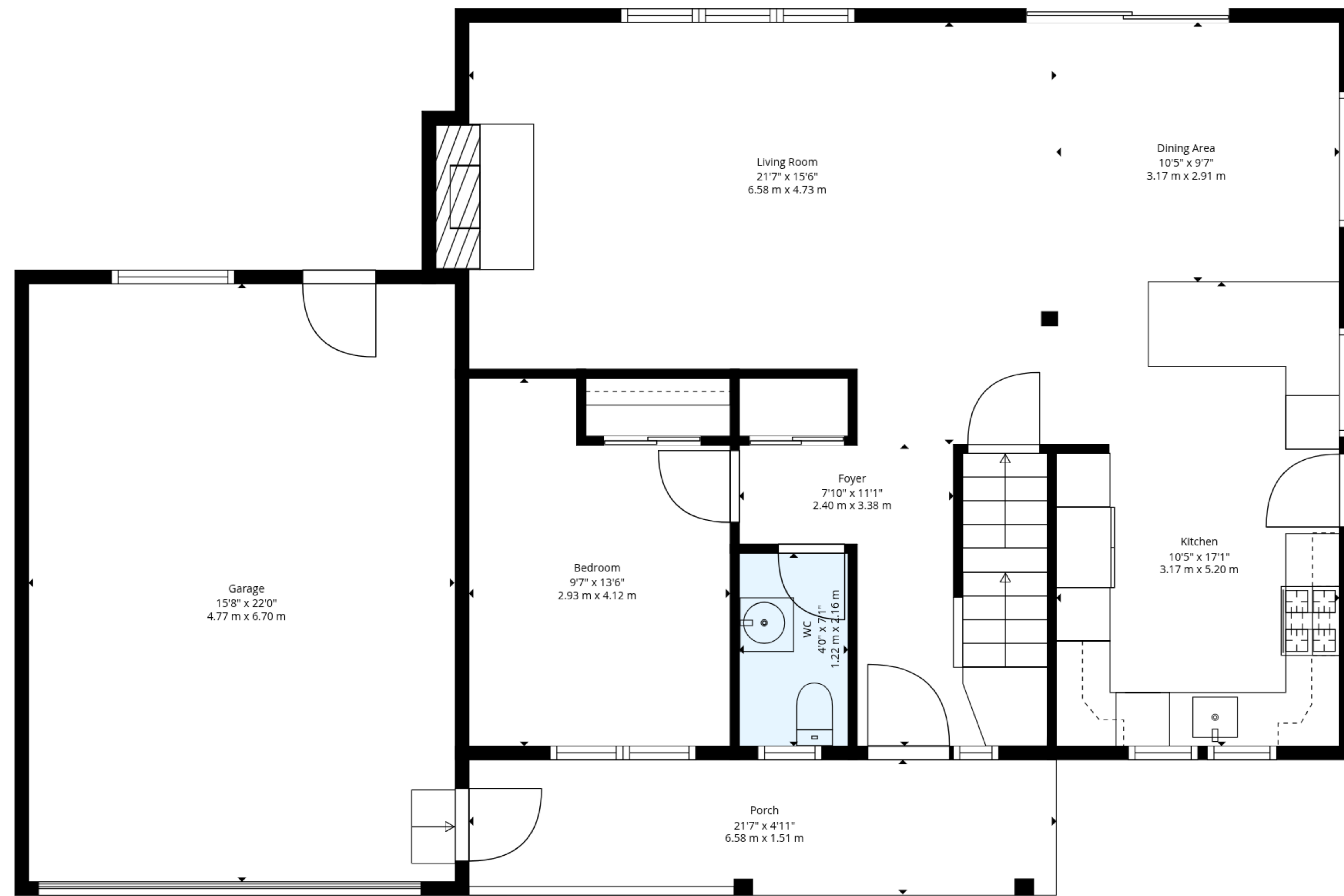
Ground Floor
