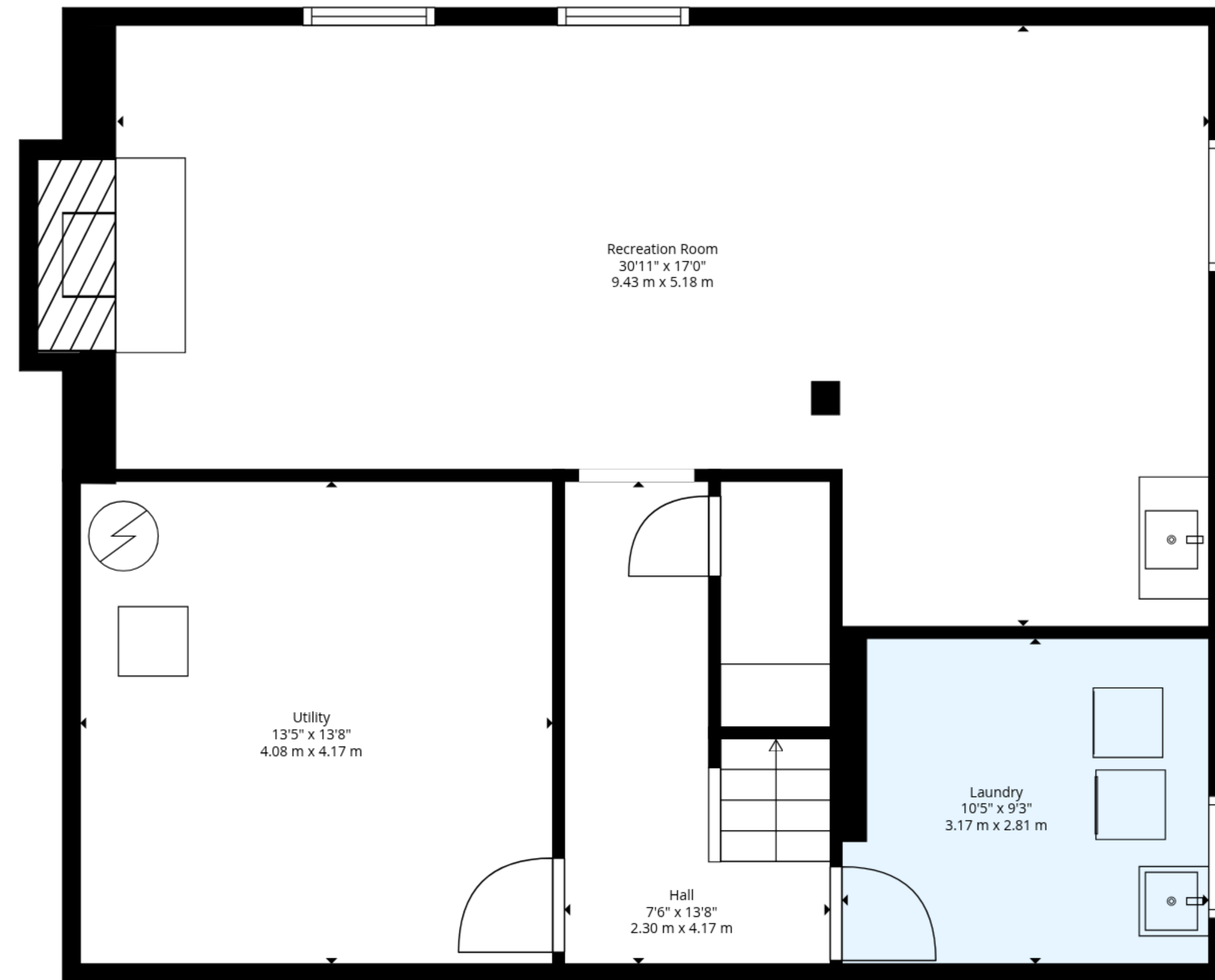
Basement
