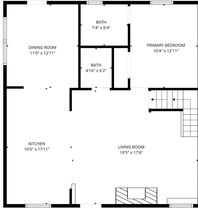
1st floor
