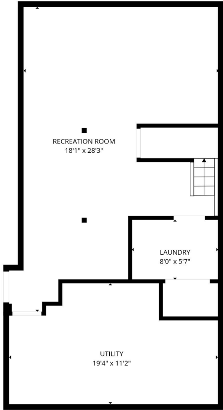
Basement
