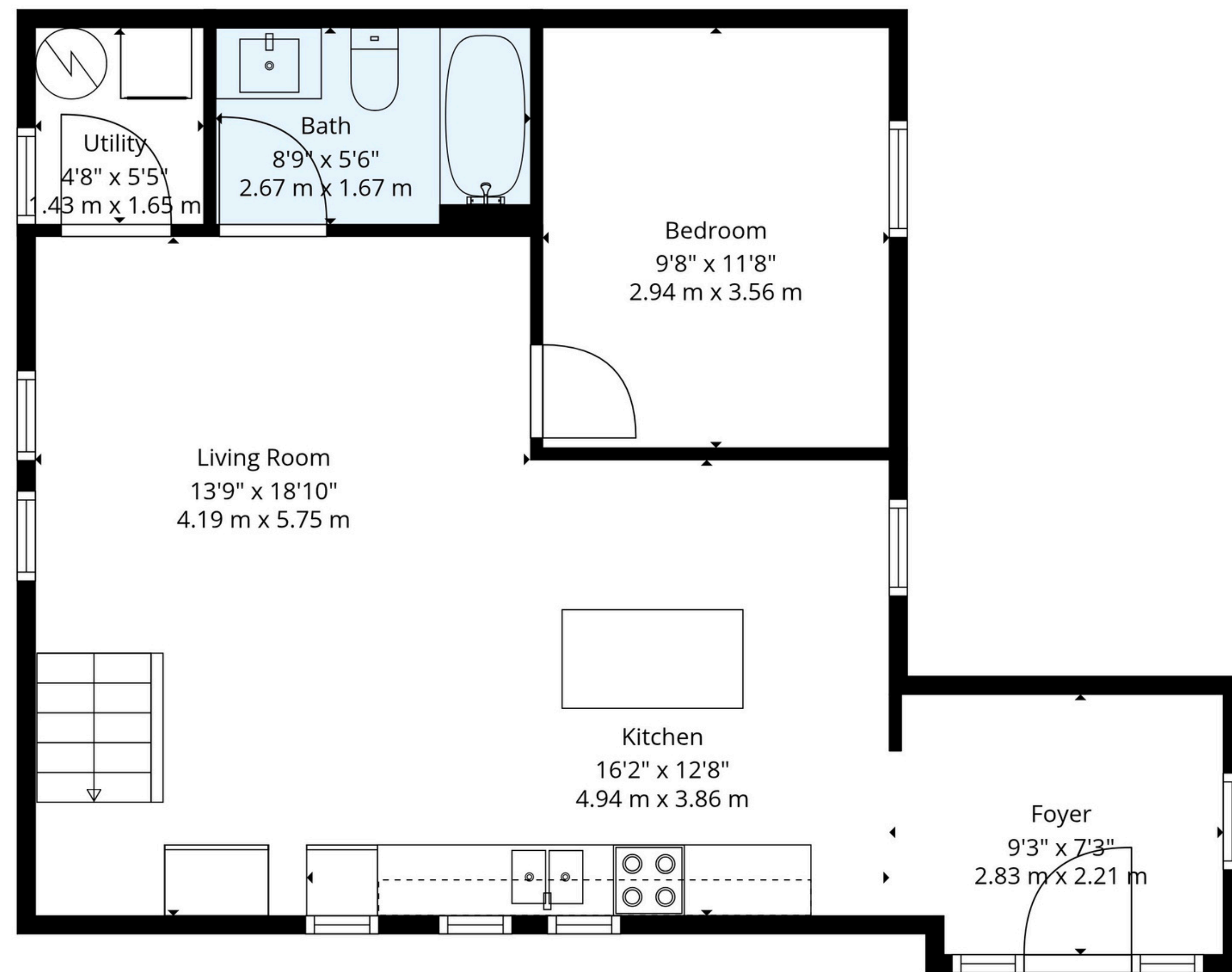
Unit 1 Ground Floor
