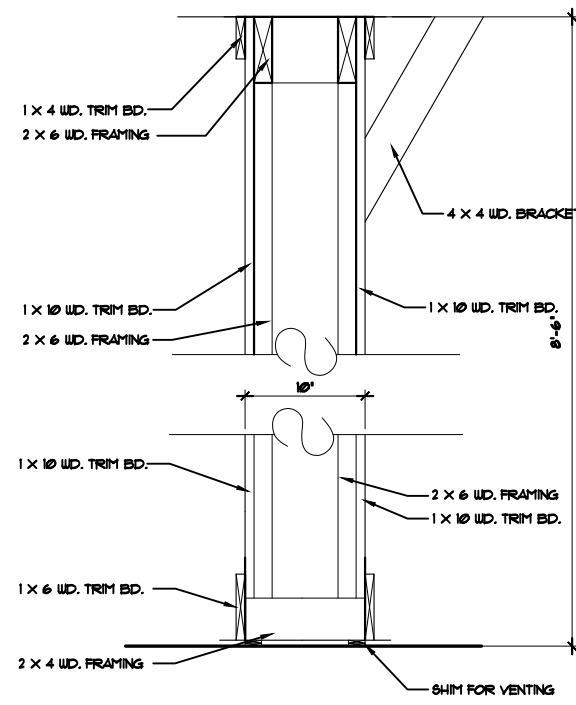
10" X 10" WD. BUILT-UP COLUMN SCALE: 3/4" = 1'-0"
