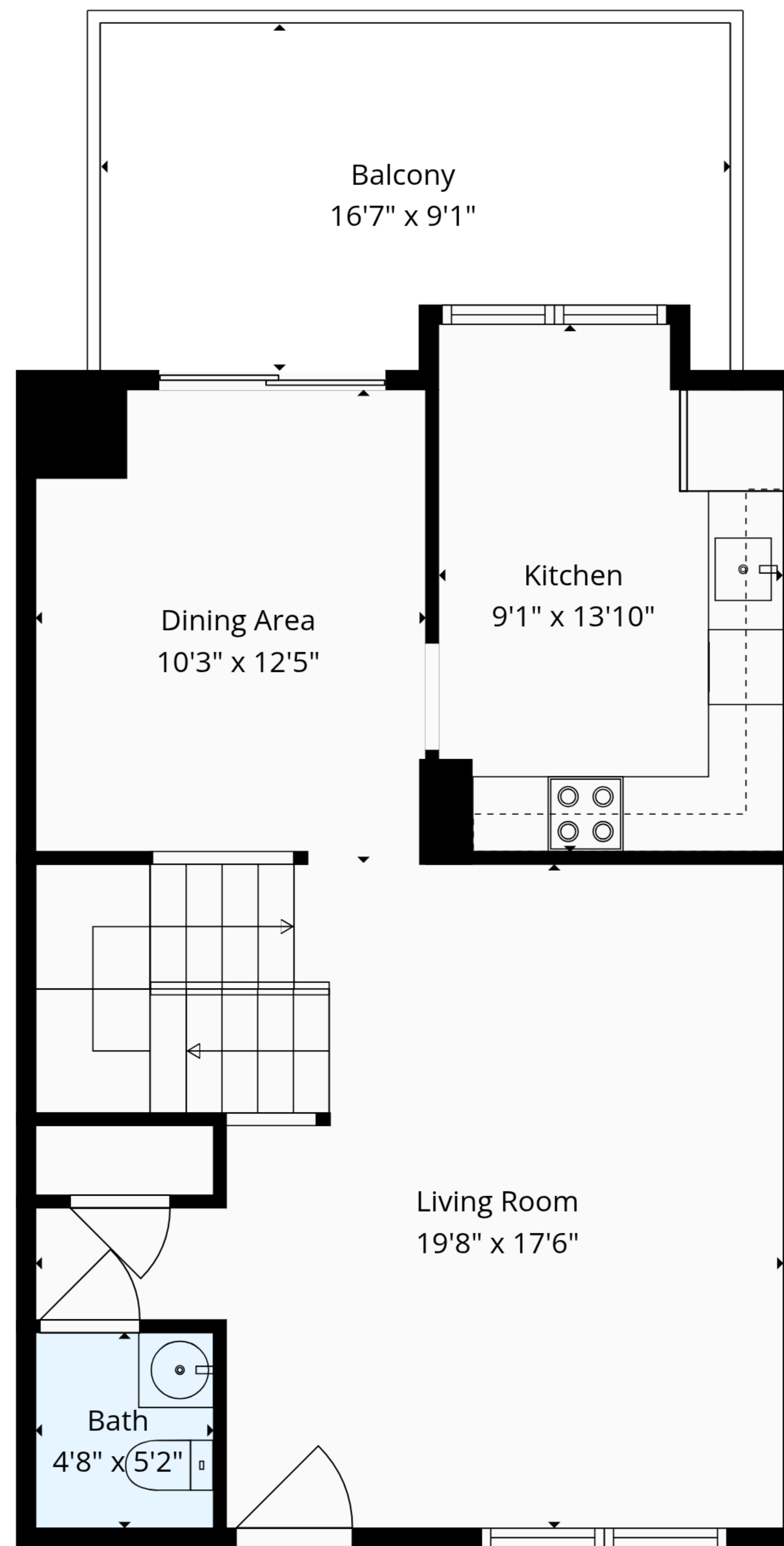
1st Floor
