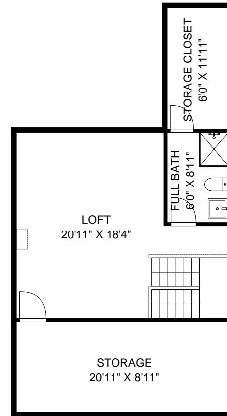
THIRD FLOOR
