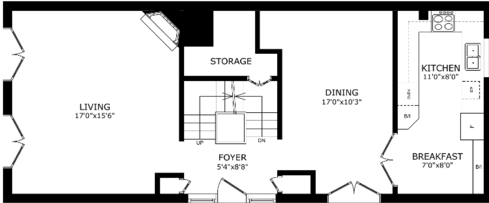
MAIN FLOOR
