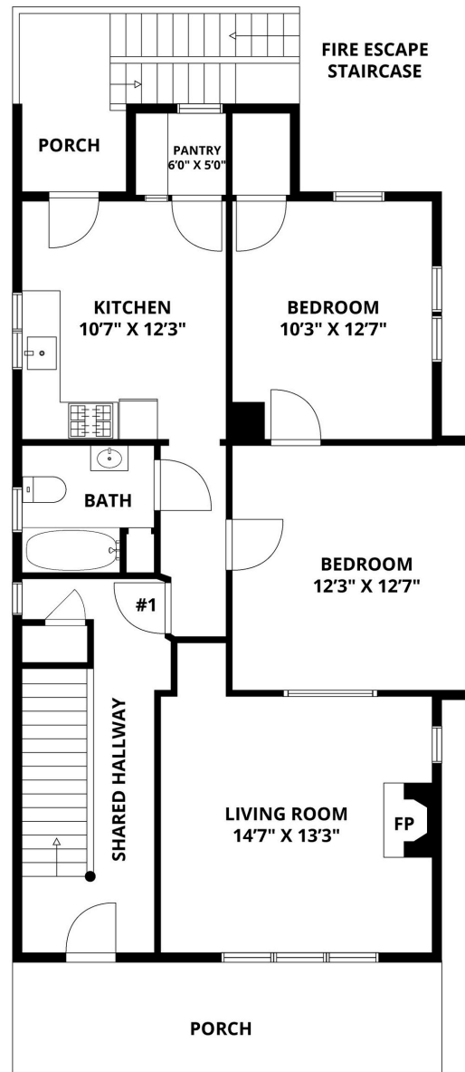
GROUND FLOOR APT 1
