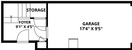
BASEMENT
