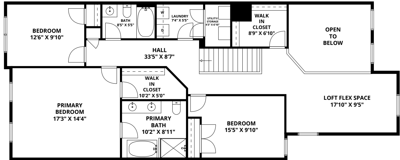
SECOND FLOOR
