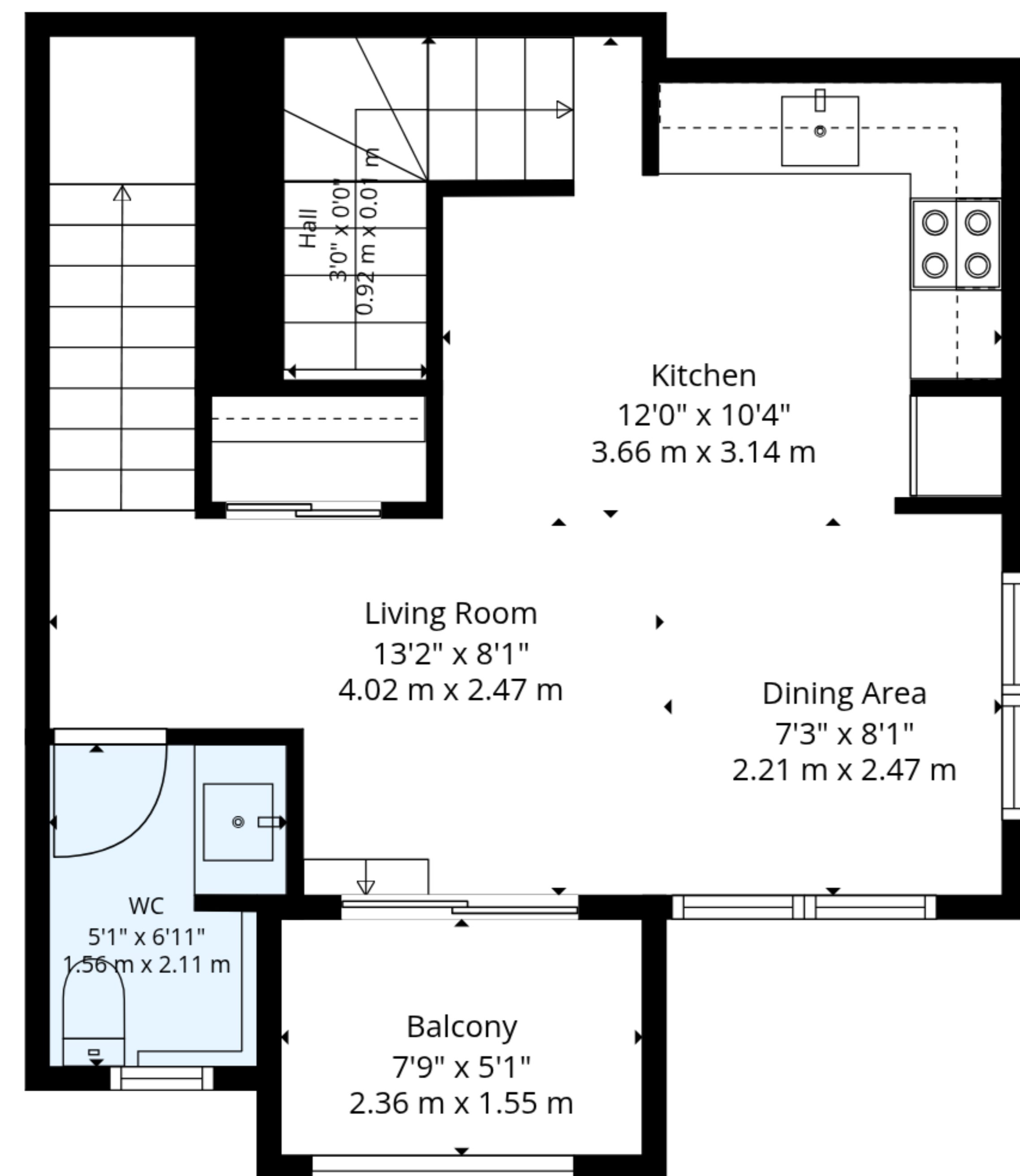
Ground Floor
