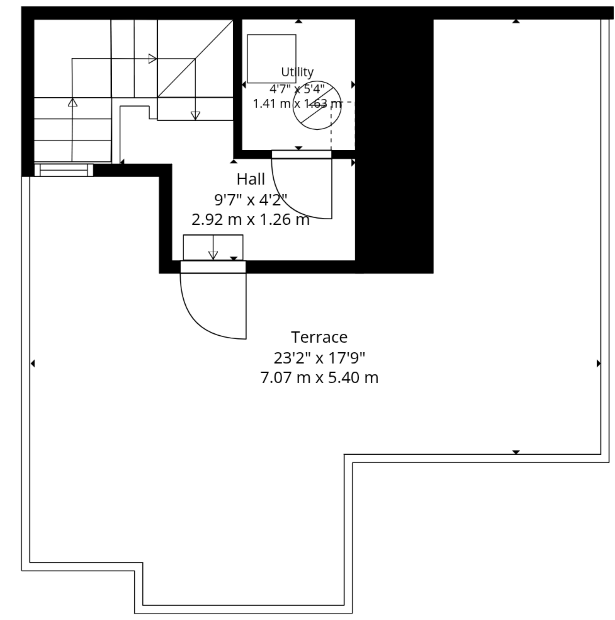
2nd Floor
