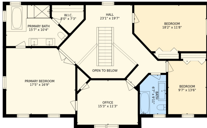
2ND FLOOR
