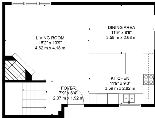
FLOOR 2
