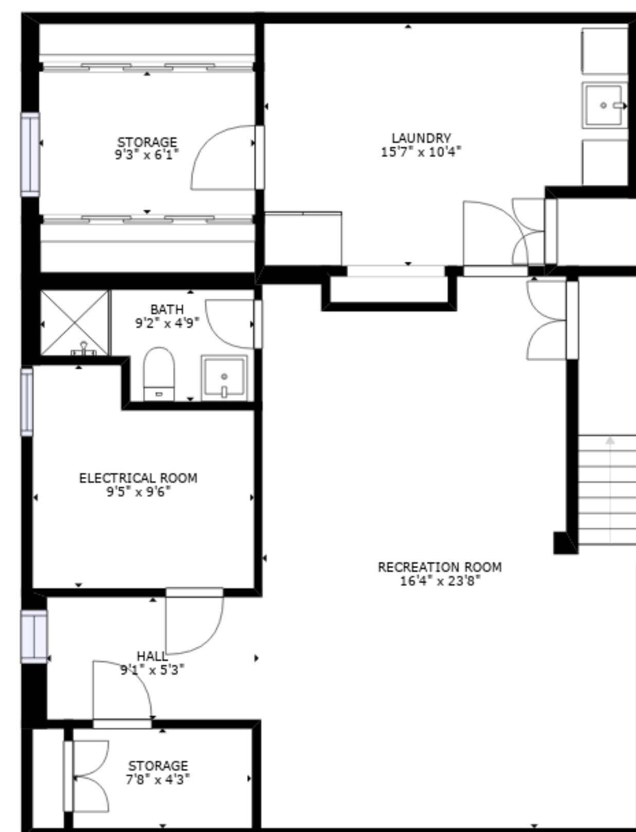
FLOOR 1
