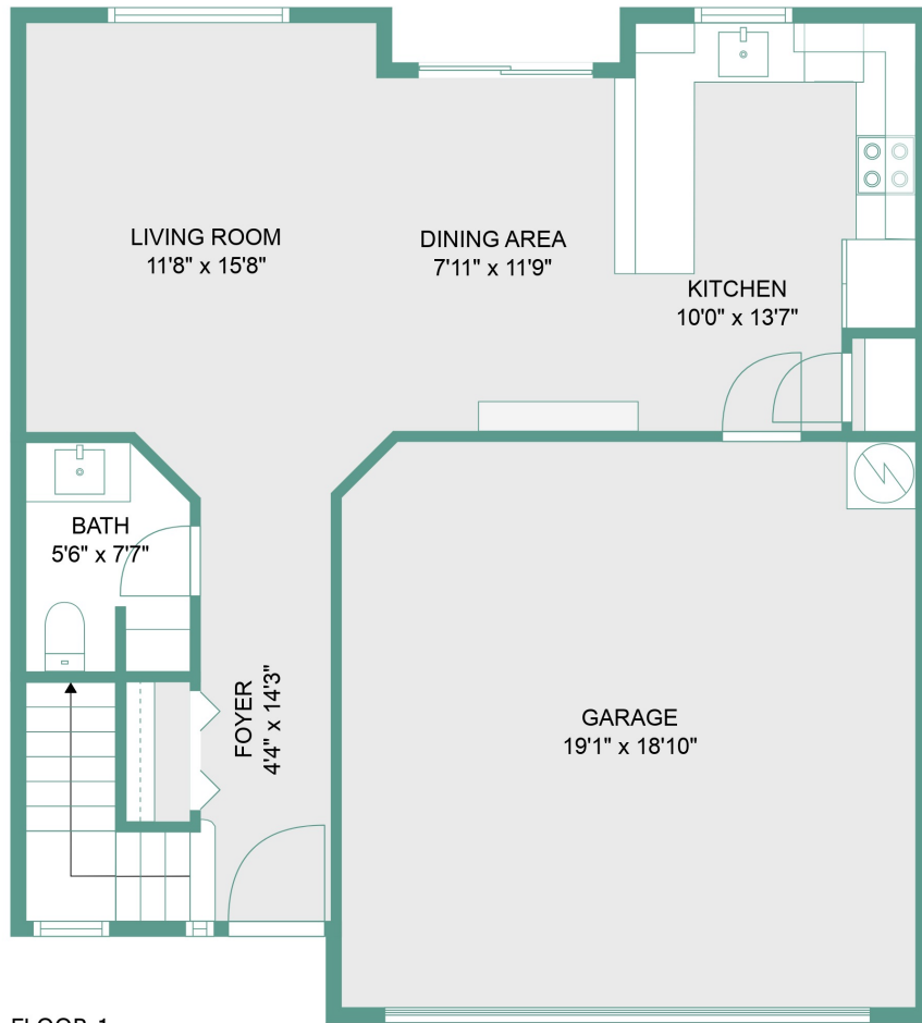
FLOOR 1
